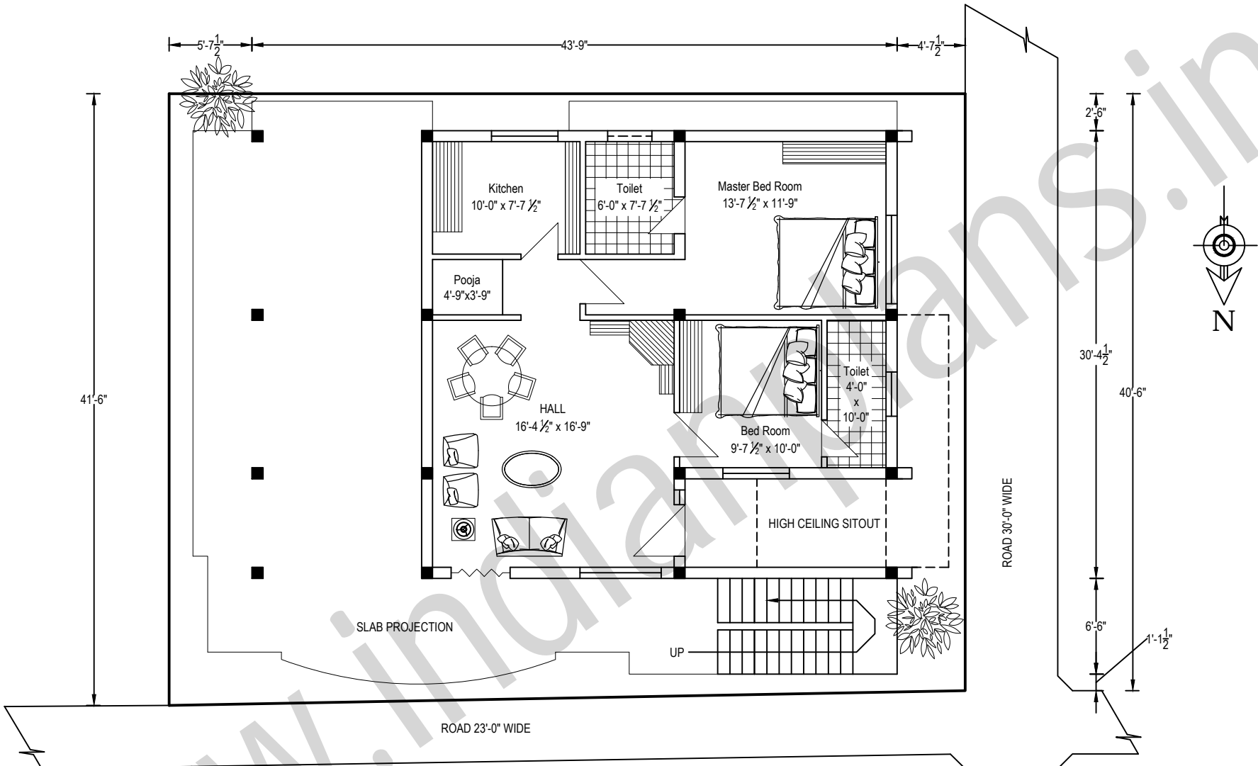
PROPOSED GROUND FLOOR RESIDENTIAL BUILDING
